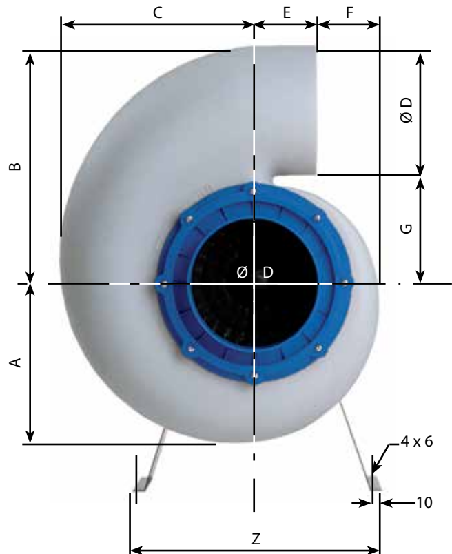
CCW POSITION
