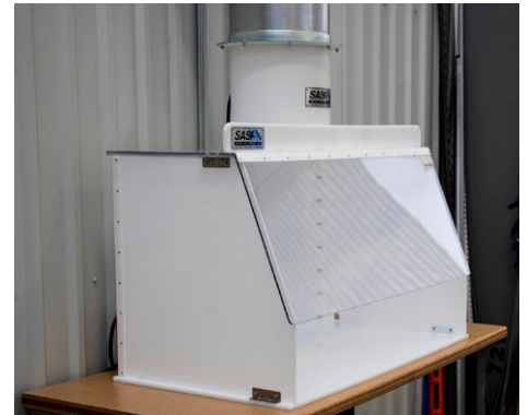
The 40" Powered Exhaust Hood with Inline Fan pulls most of the harmful fumes away from the operator's breathing zone.
