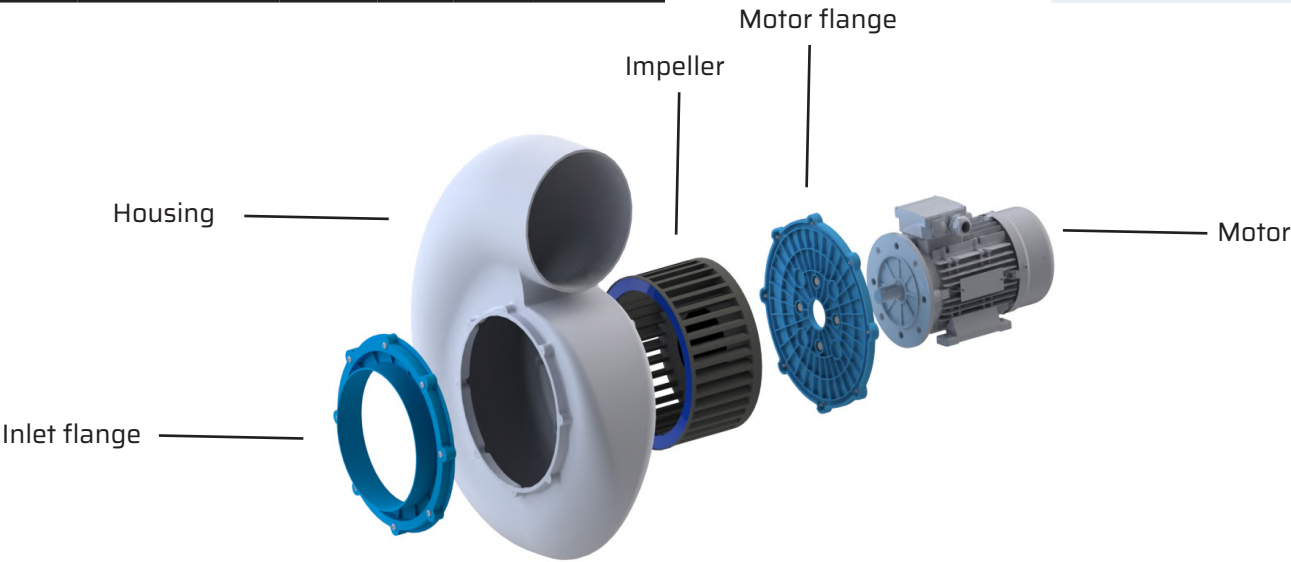
Exploded view
