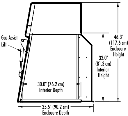
SIDE (4', 5', 6' MODELS, TALL & DEEP)
