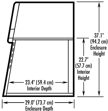
SIDE (2', 3', 4' MODELS)
