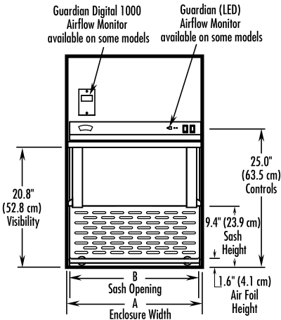
FRONT (2', 3', 4' MODELS)
